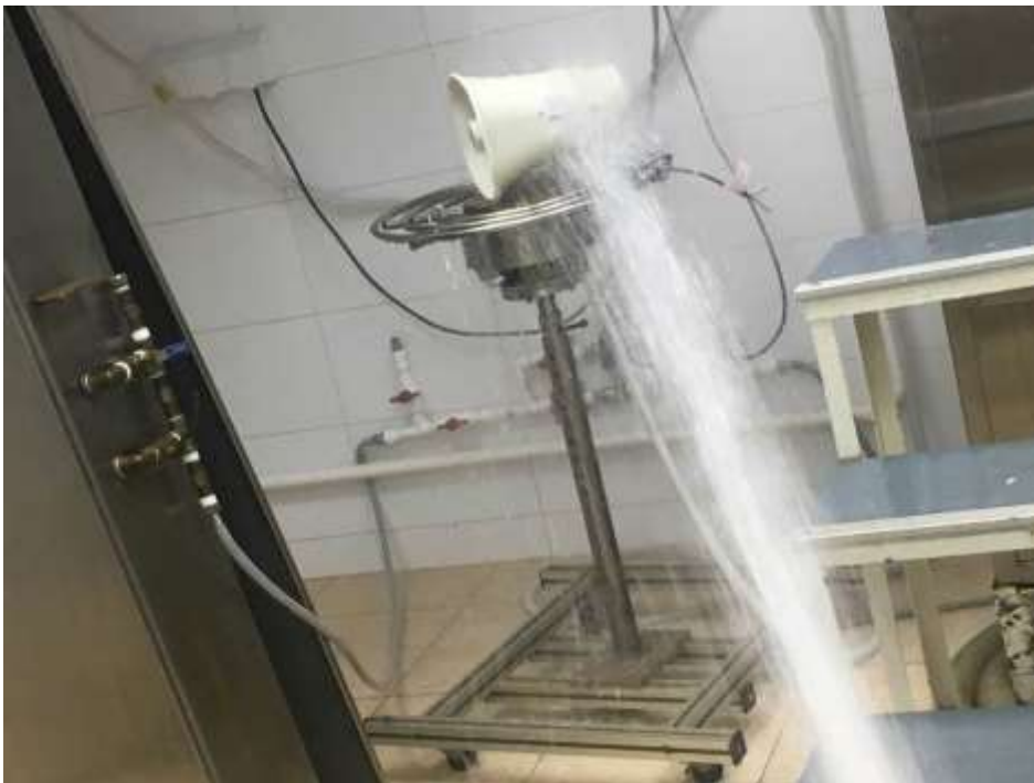
Picture 10 (Sample after the IPX6 test)
