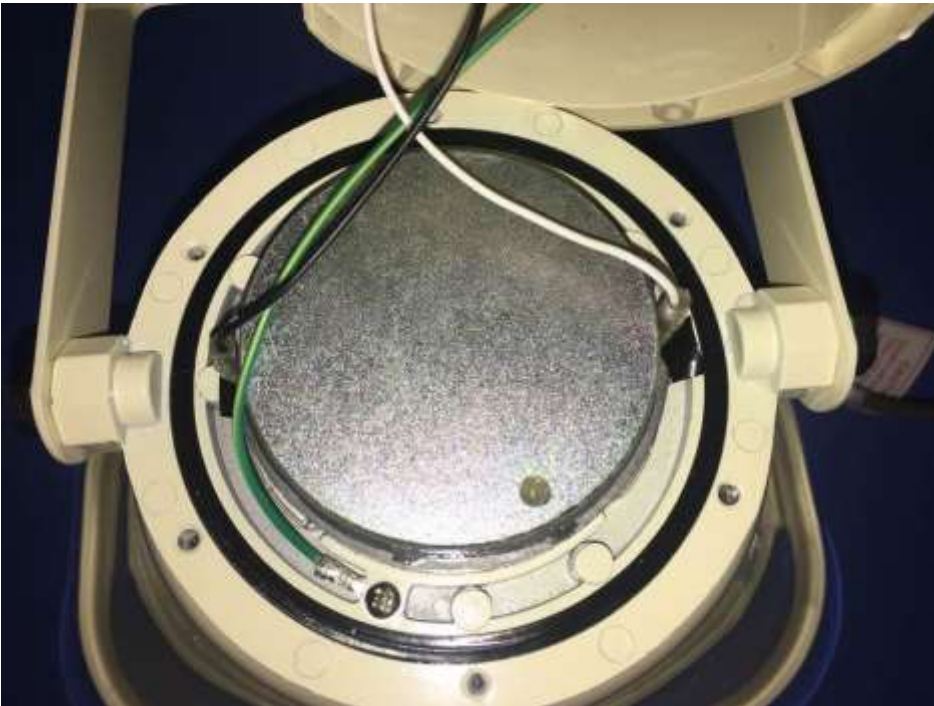
Picture 14 (Sample for the IPX6 test)
